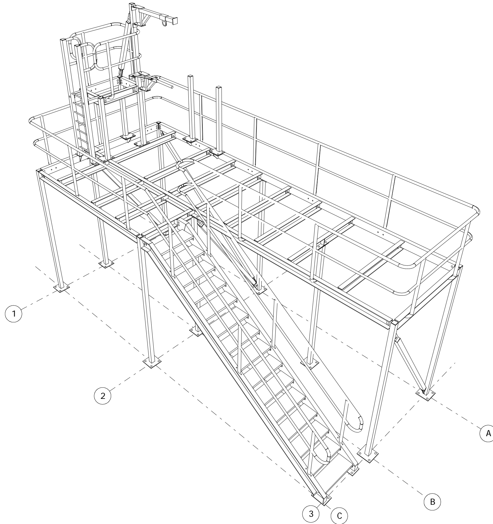
3-D VIEW
